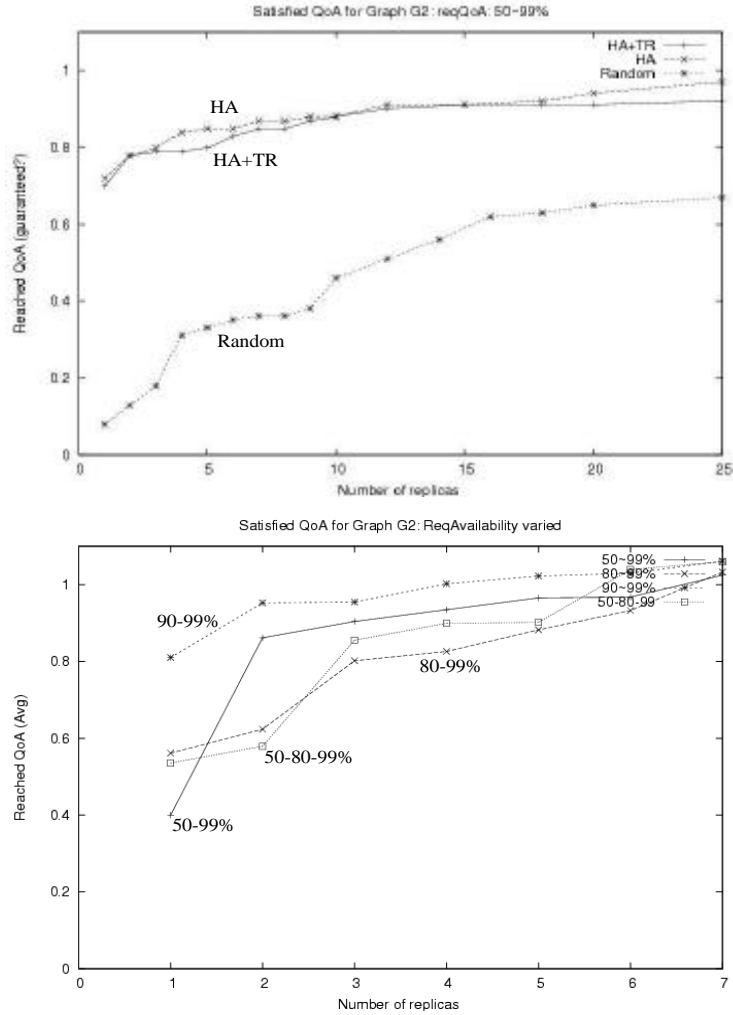
Figure 3: Reached QoA values by our heuristics: (top) different heuristics, (bottom) different ranges for required availability values
