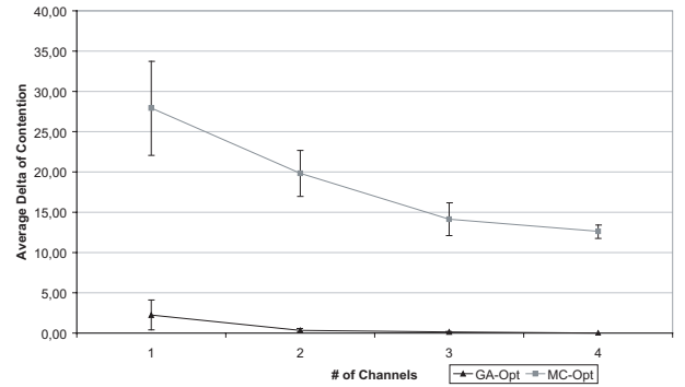
Figure 1: Average of pairwise differences between GA and solver as well as between MC and solver, with 95% confidence interval.
